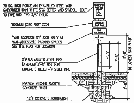
ACCESS PARKING SIGN NOT TO SCALE
