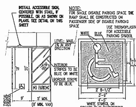
ACCESS PARKING AND SYMBOL NOT TO SCALE
