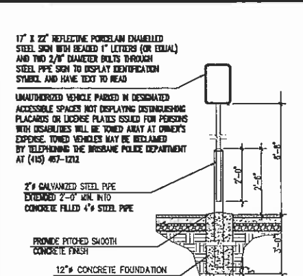
SITE ENTRY ACCESS PARKING SIGN NOT TO SCALE
